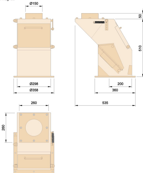
Ard Machine Flat Magnetic Separator
